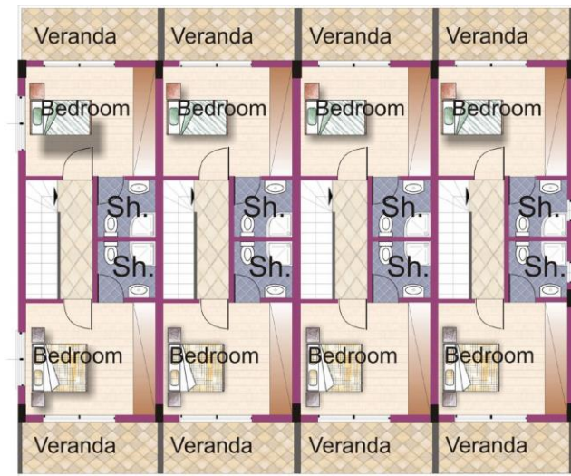
FRST FLOOR
